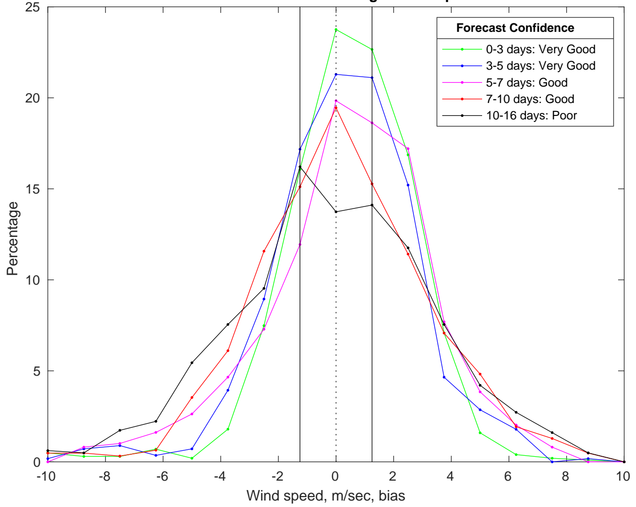
NDBC 42035 vs GFS Winds Bias Histogram: 04-Apr-2025
