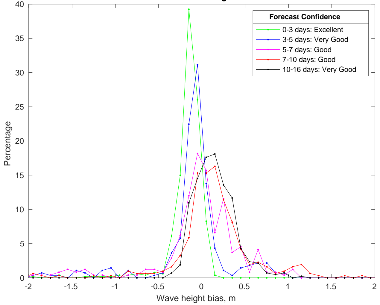
NDBC 42035 vs GFSWave Bias Histogram: 20-Jul-2024
