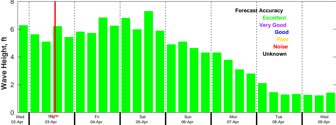
AUSWAV Wave Forecast for NDBC 42035 from 02-Apr-2025 18:00:00 to 09-Apr-2025 18:00:00
