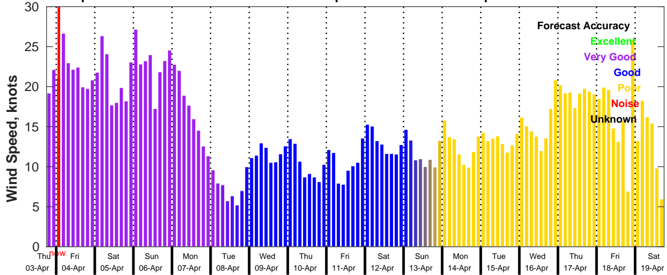
GFS Wind Speed Forecast for NDBC 42035 from 03-Apr-2025 18:00:00 to 19-Apr-2025 18:00:00
