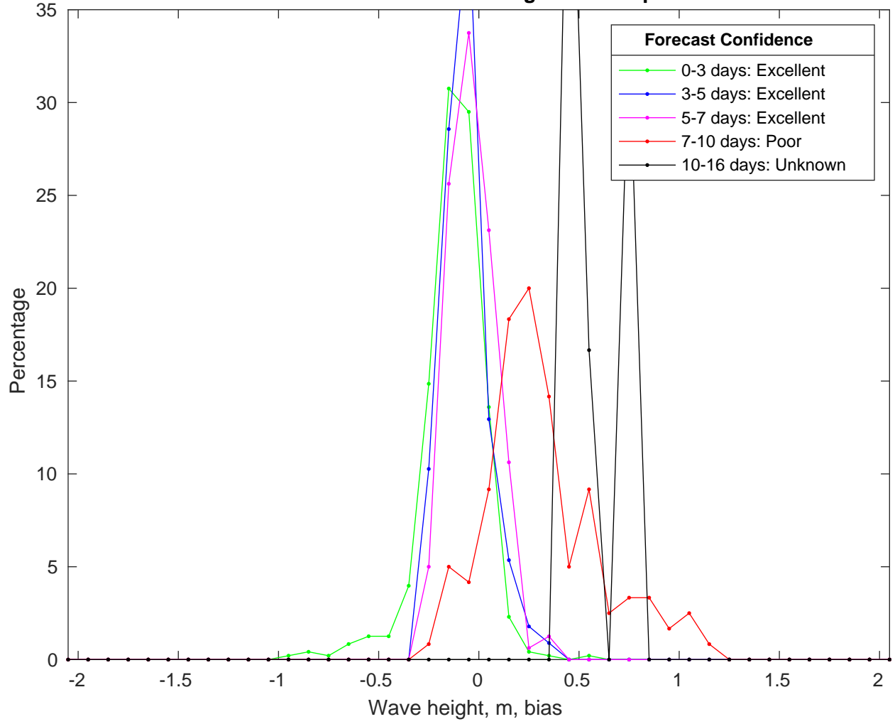
NDBC 42035 vs GFSWaves Bias Histogram: 19-Sep-2024
