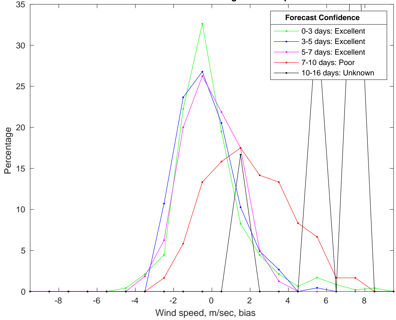
NDBC 42035 vs GFSWinds Bias Histogram: 19-Sep-2024
