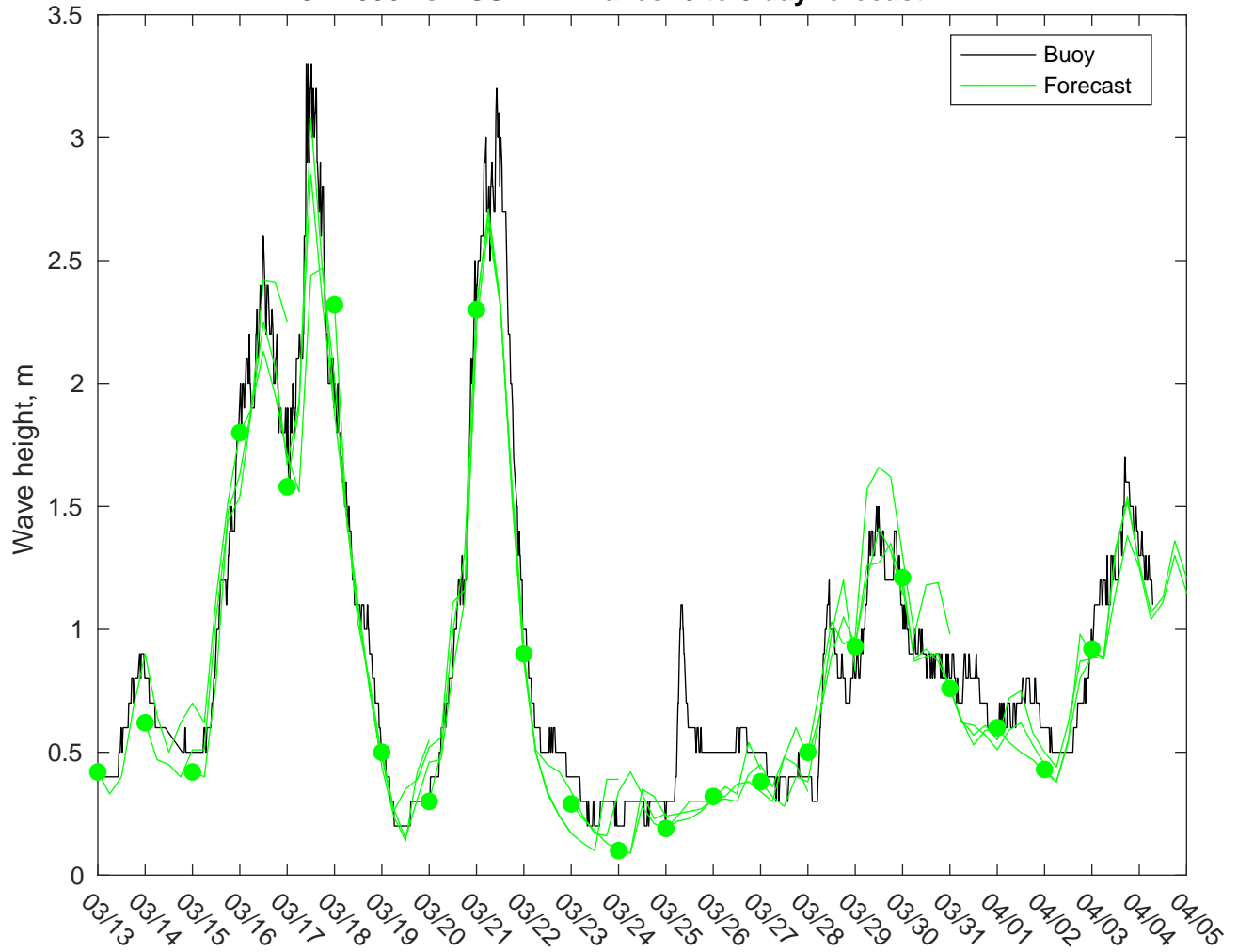
NDBC 42036 vs AUSWAV Waves: 0 to 3 day forecast
