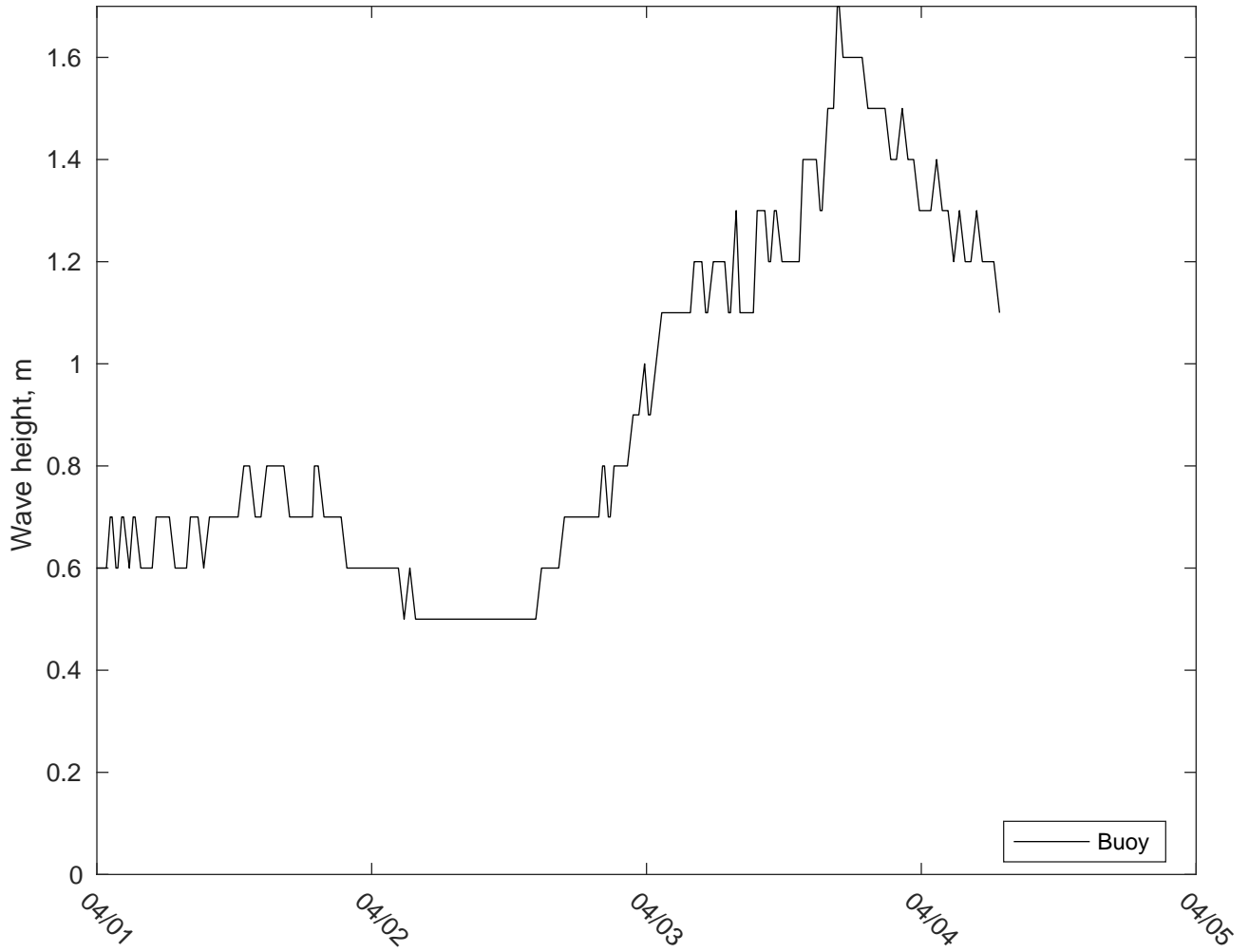
NDBC 42036 vs AUSWAV Waves: 7 to 10 day forecast
