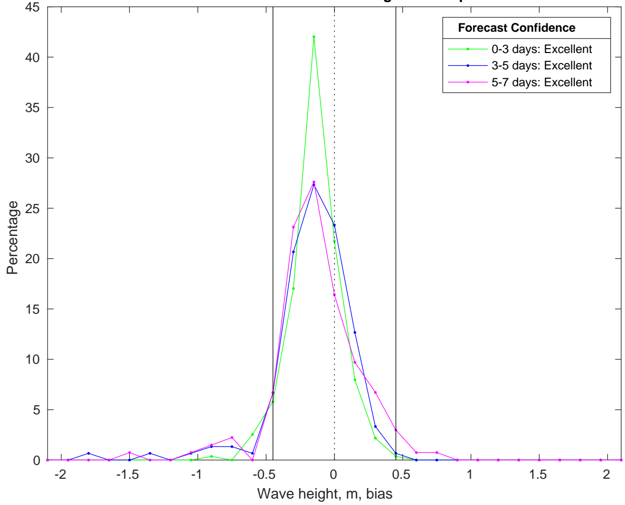
NDBC 42036 vs AUSWAV Waves Bias Histogram: 04-Apr-2025
