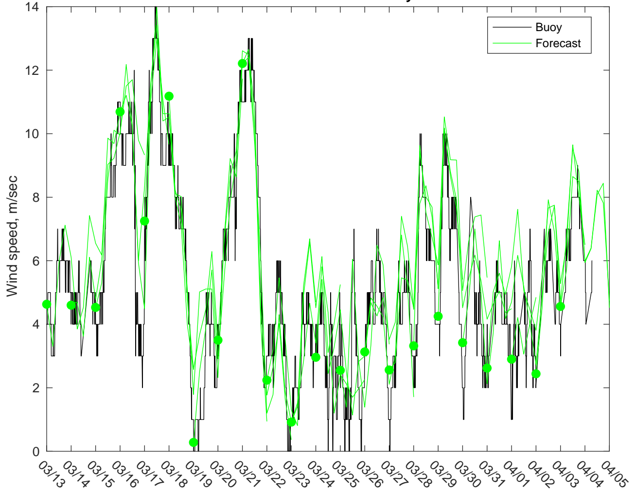
NDBC 42036 vs AUSWAV Winds: 0 to 3 day forecast
