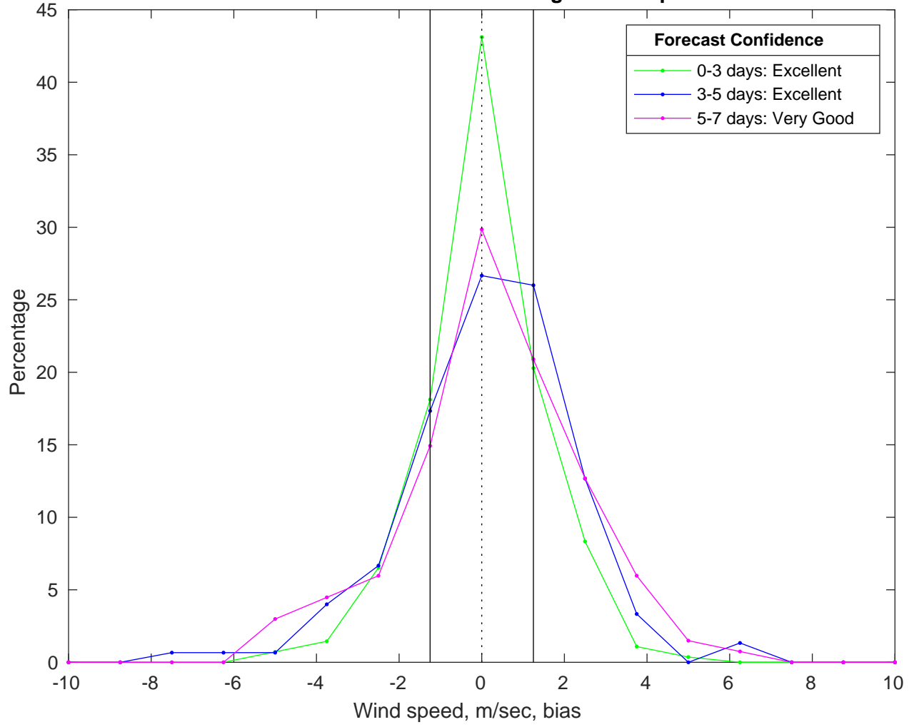
NDBC 42036 vs AUSWAV Winds Bias Histogram: 04-Apr-2025
