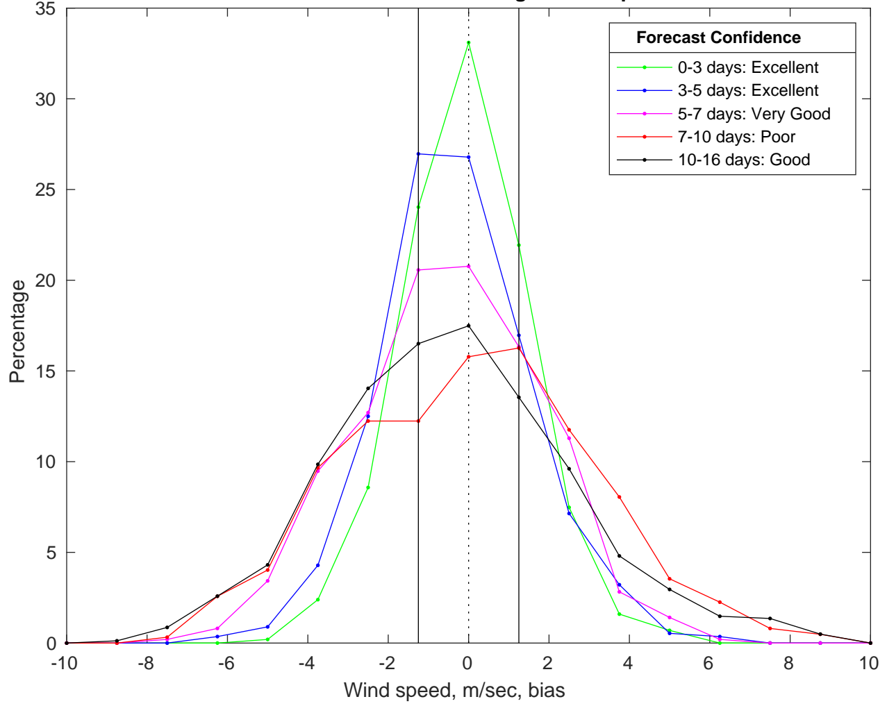
NDBC 42036 vs GFS Winds Bias Histogram: 04-Apr-2025
