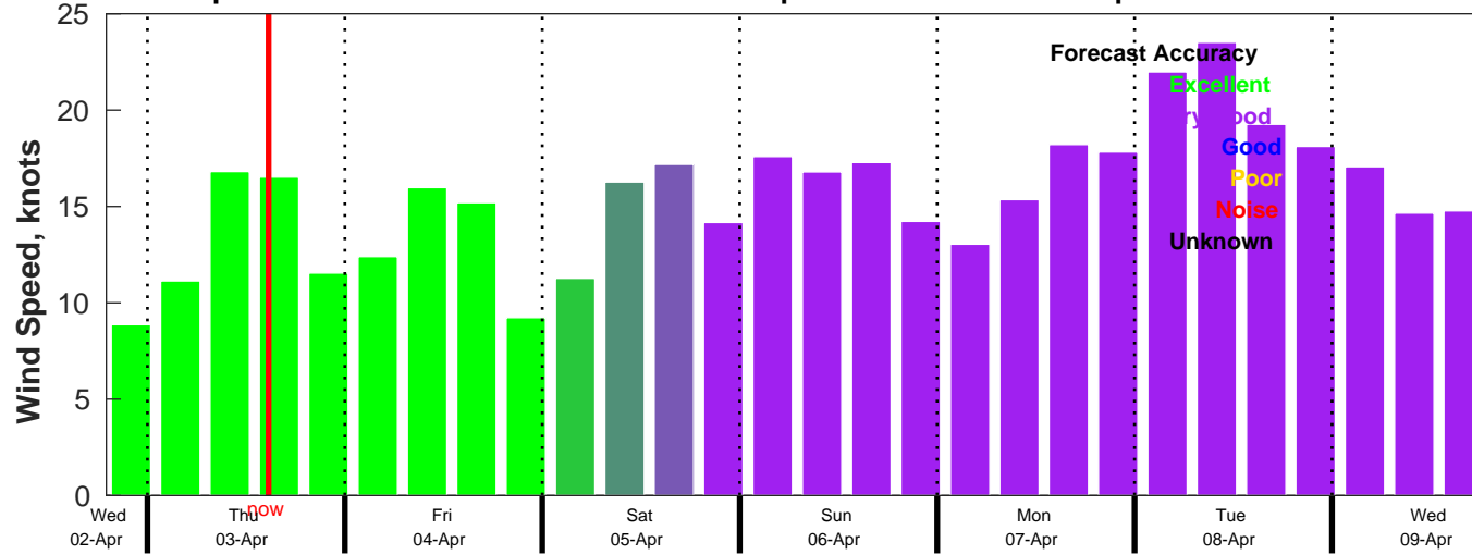
AUSWAV Wind Speed Forecast for NDBC 42036 from 02-Apr-2025 19:00:00 to 09-Apr-2025 19:00:00
