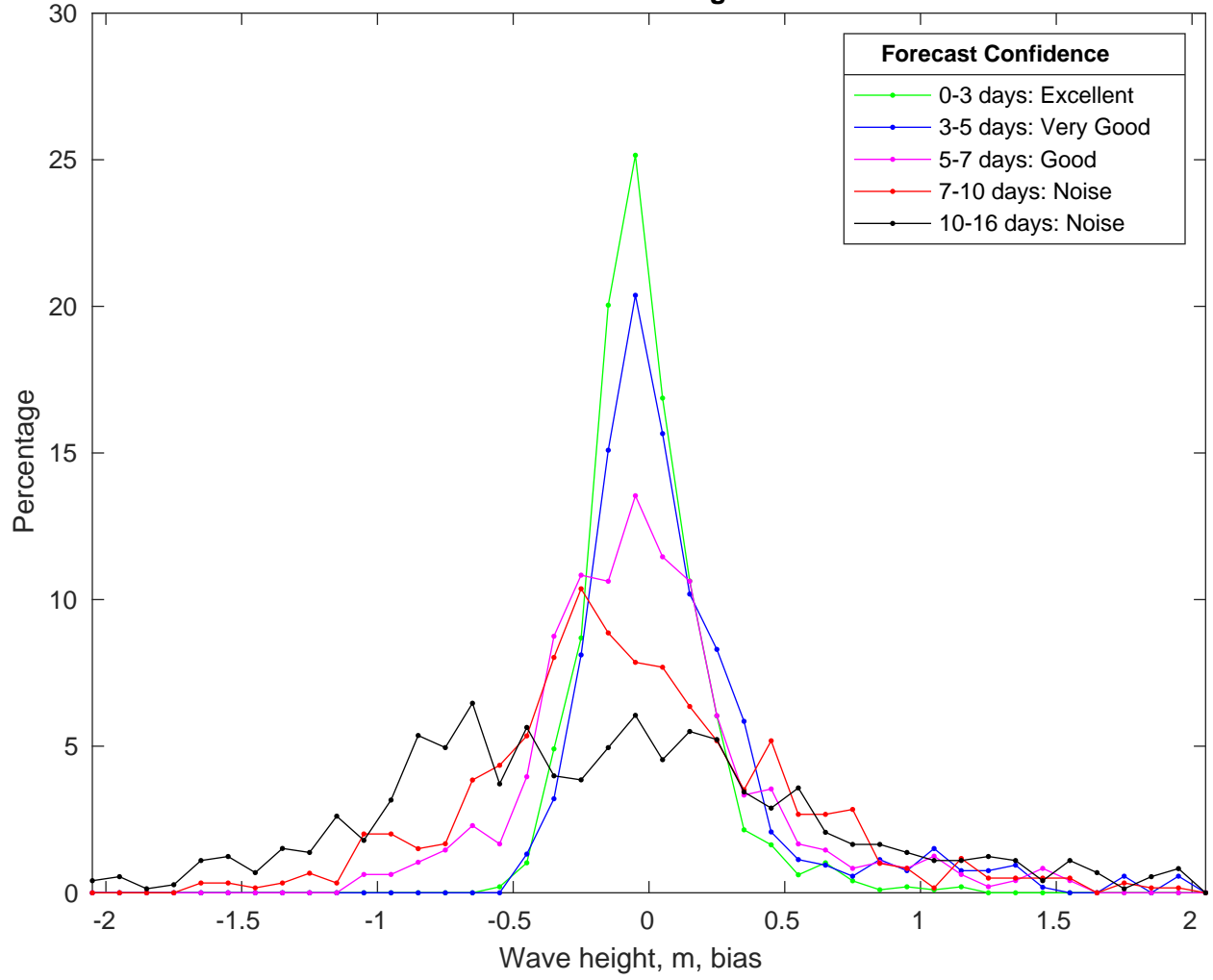
NDBC 42036 vs GFSWaves Bias Histogram: 12-Nov-2024
