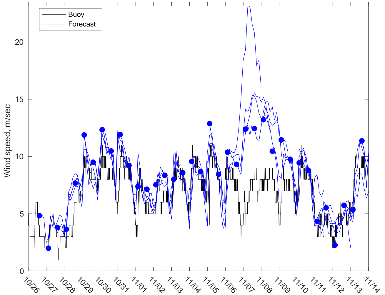
NDBC 42036 vs GFSWinds: 3 to 5 day forecast
