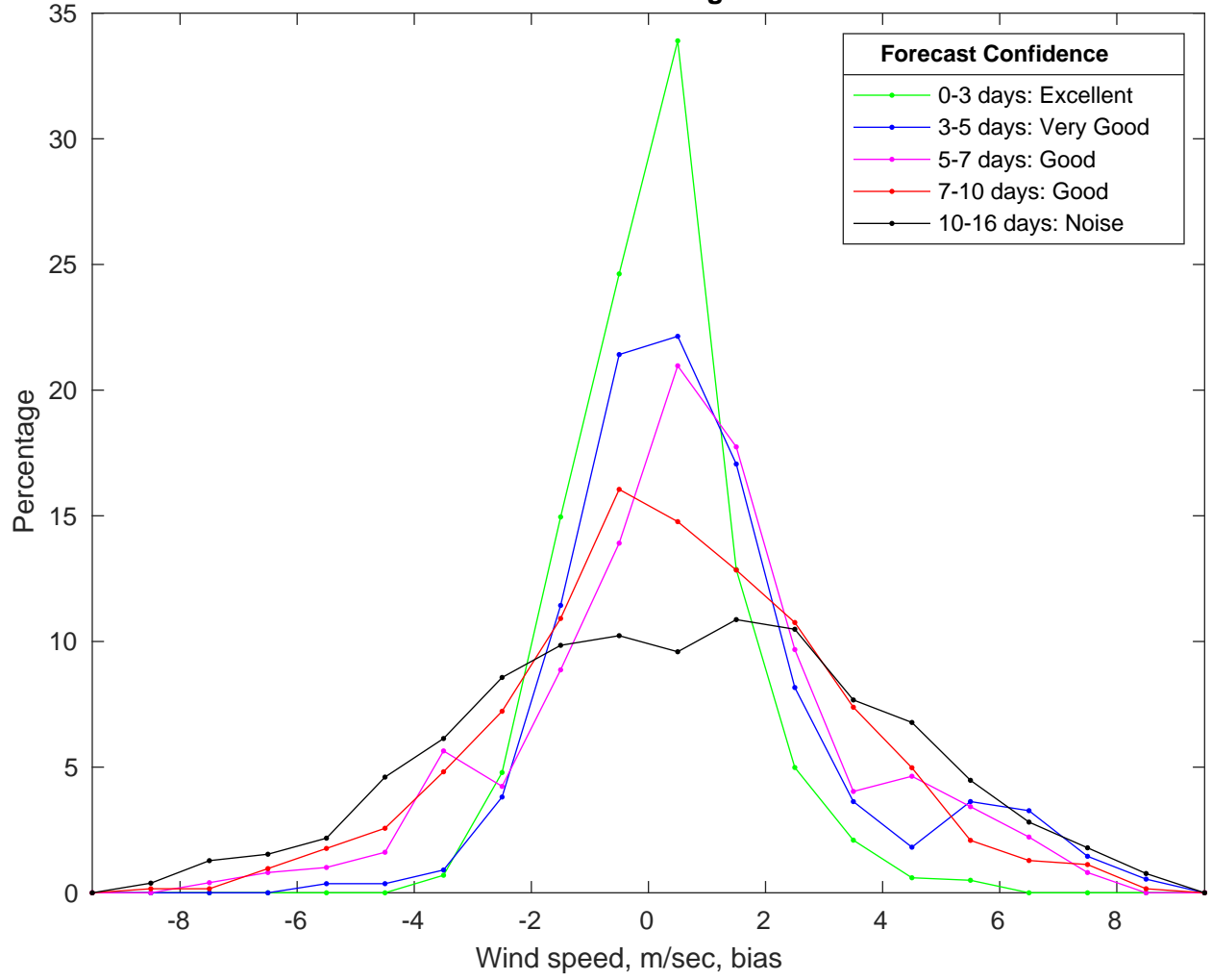
NDBC 42036 vs GFSWinds Bias Histogram: 13-Nov-2024
