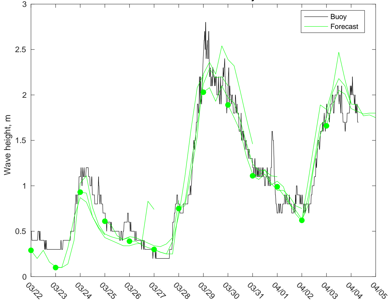
NDBC 42040 vs AUSWAV Waves: 0 to 3 day forecast
