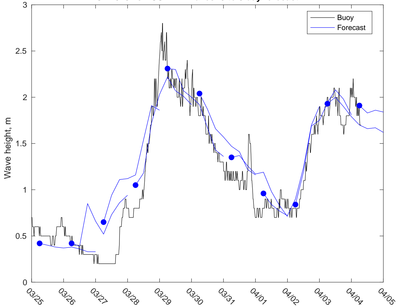
NDBC 42040 vs AUSWAV Waves: 3 to 5 day forecast
