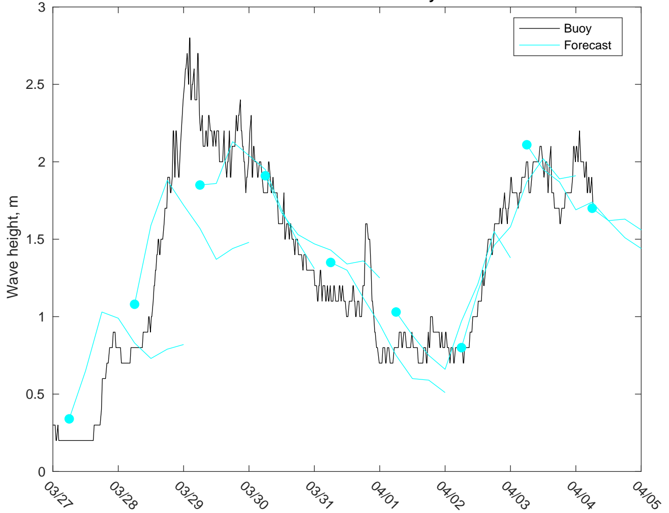
NDBC 42040 vs AUSWAV Waves: 5 to 7 day forecast
