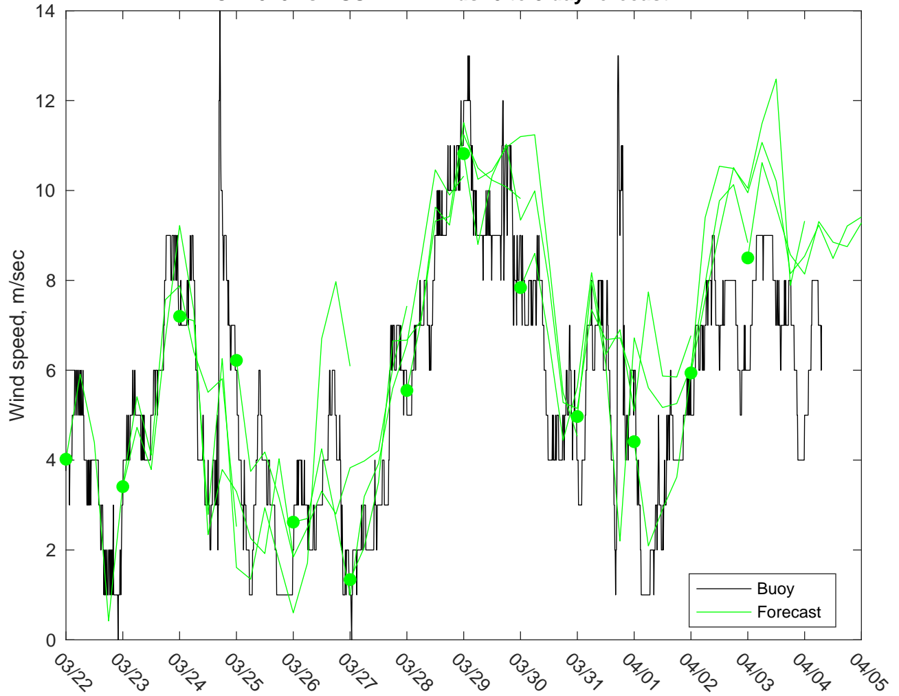
NDBC 42040 vs AUSWAV Winds: 0 to 3 day forecast
