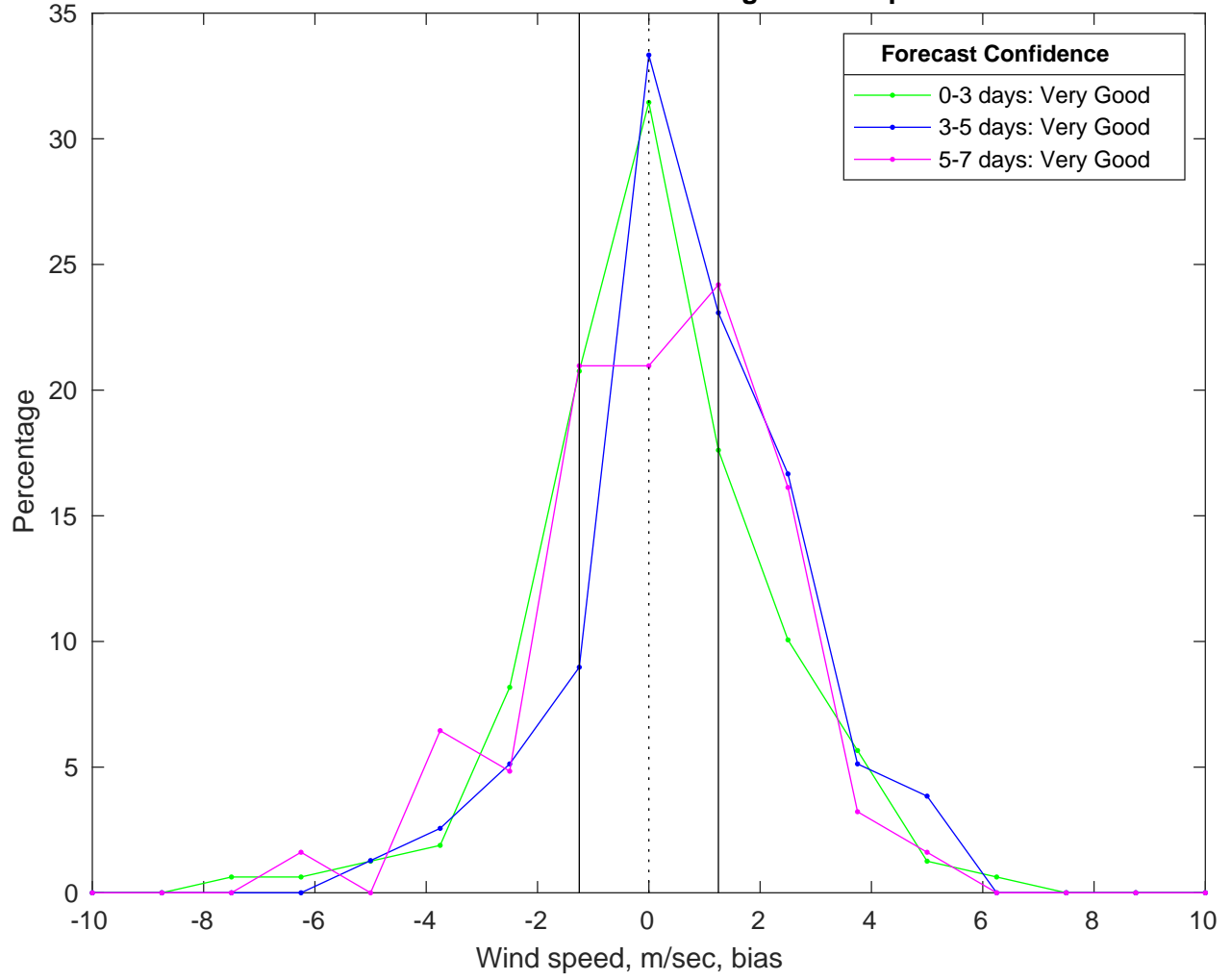
NDBC 42040 vs AUSWAV Winds Bias Histogram: 04-Apr-2025
