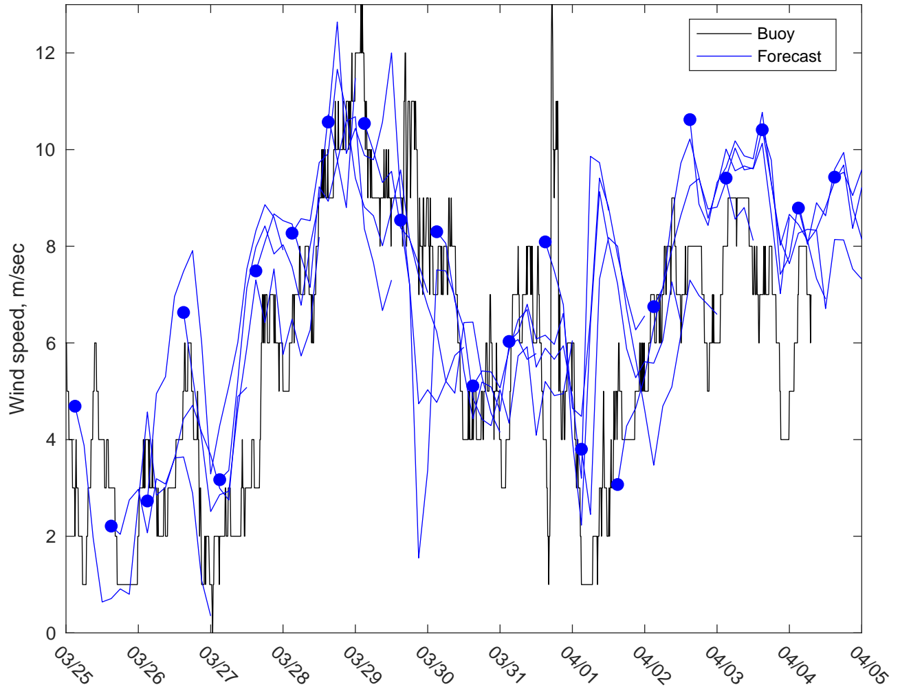
NDBC 42040 vs GFS Winds: 3 to 5 day forecast
