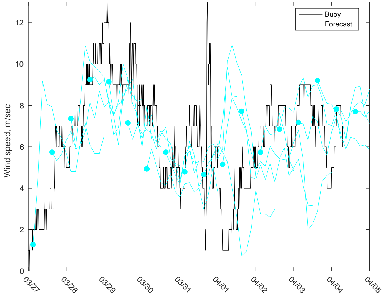
NDBC 42040 vs GFS Winds: 5 to 7 day forecast
