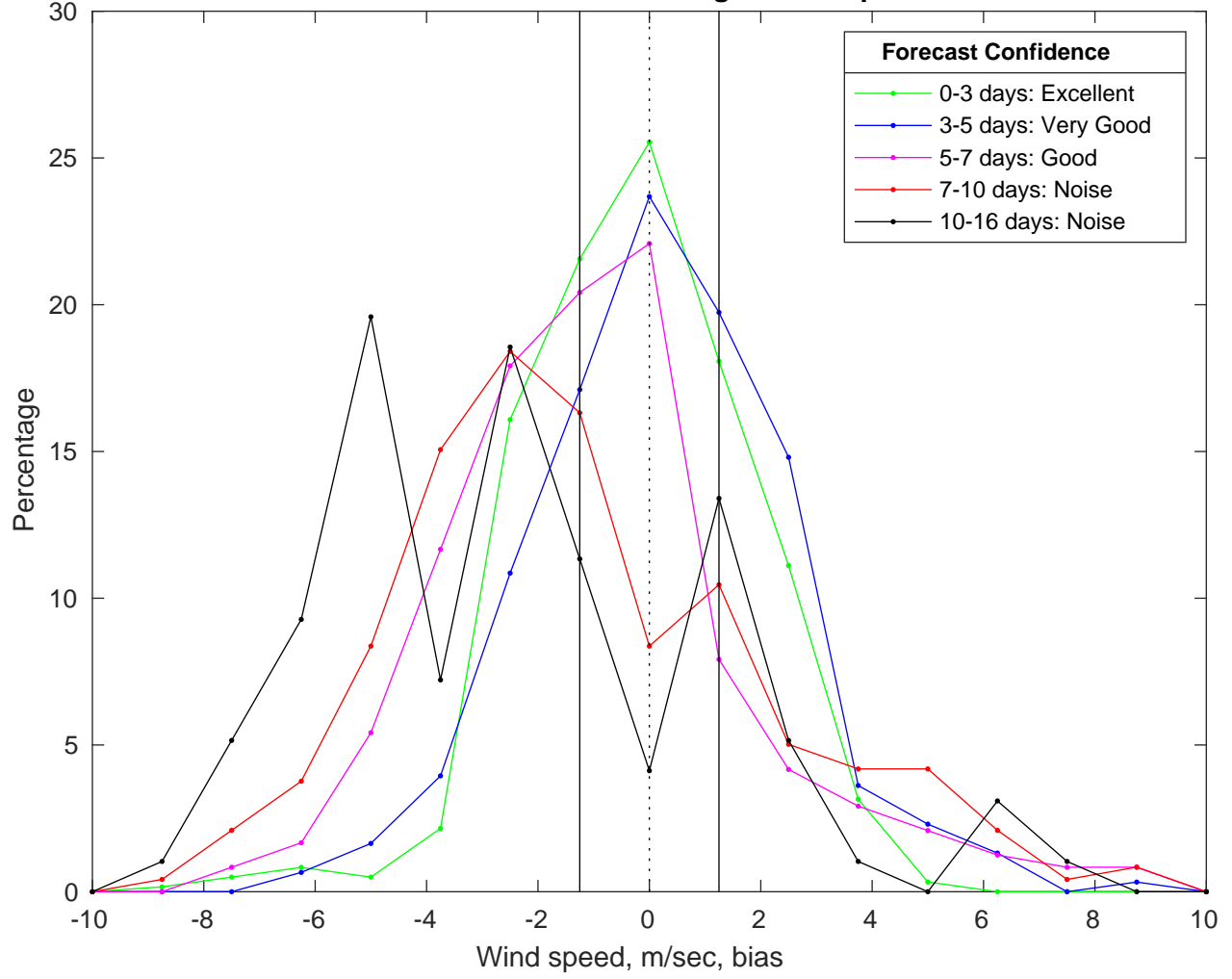
NDBC 42040 vs GFS Winds Bias Histogram: 04-Apr-2025
