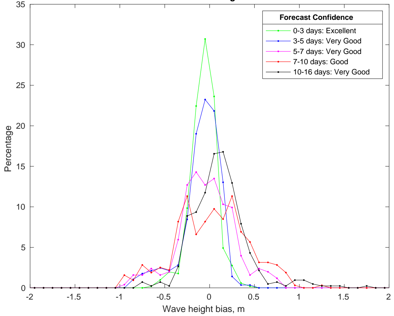
NDBC 42040 vs GFSWave Bias Histogram: 20-Jul-2024
