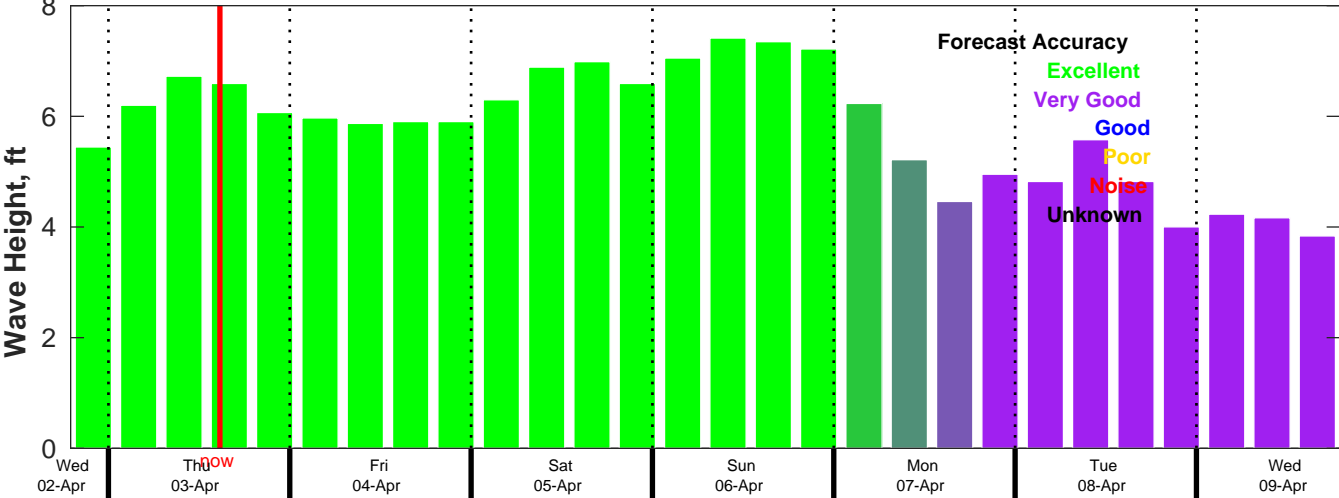
AUSWAV Wave Forecast for NDBC 42040 from 02-Apr-2025 19:00:00 to 09-Apr-2025 19:00:00
