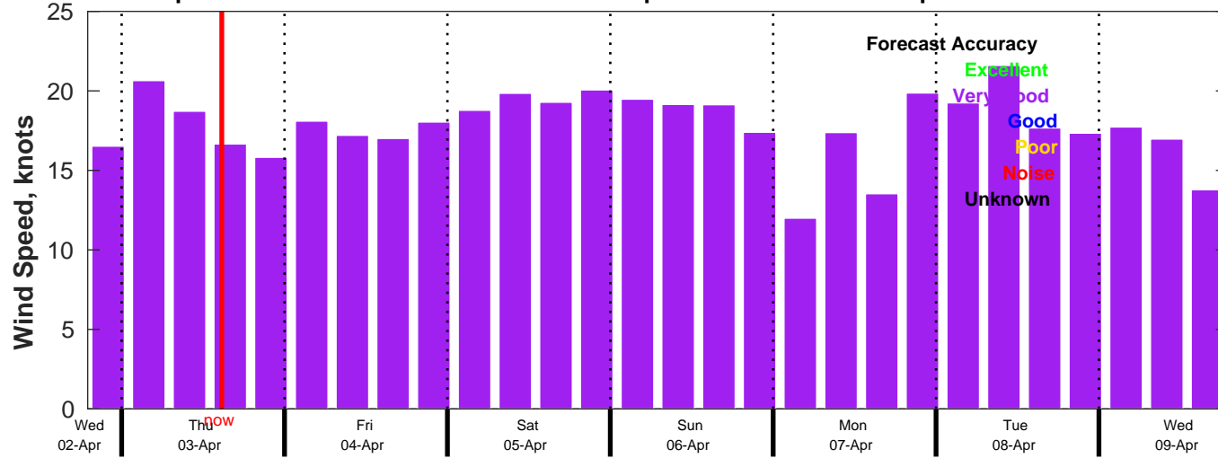
AUSWAV Wind Speed Forecast for NDBC 42040 from 02-Apr-2025 19:00:00 to 09-Apr-2025 19:00:00
