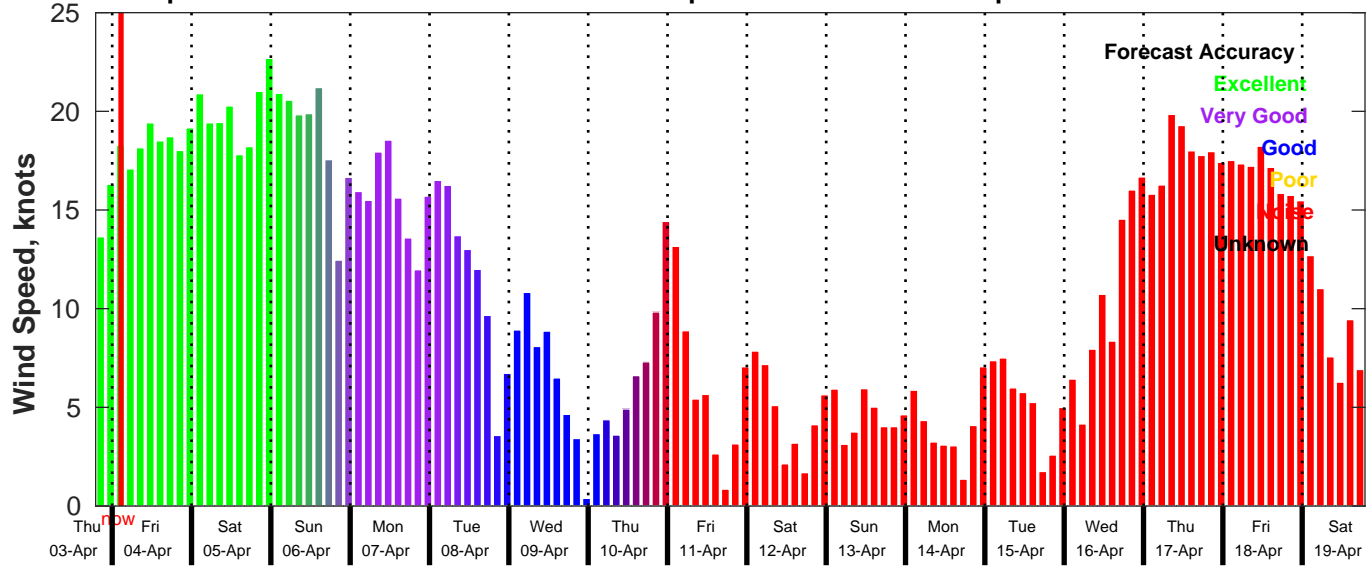
GFS Wind Speed Forecast for NDBC 42040 from 03-Apr-2025 19:00:00 to 19-Apr-2025 19:00:00
