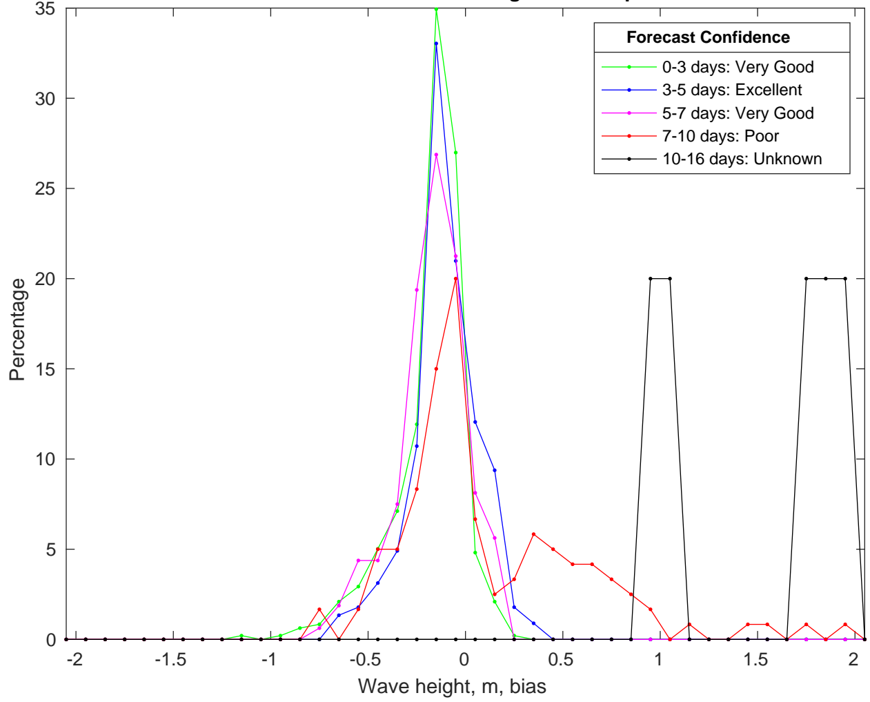
NDBC 42040 vs GFSWaves Bias Histogram: 19-Sep-2024
