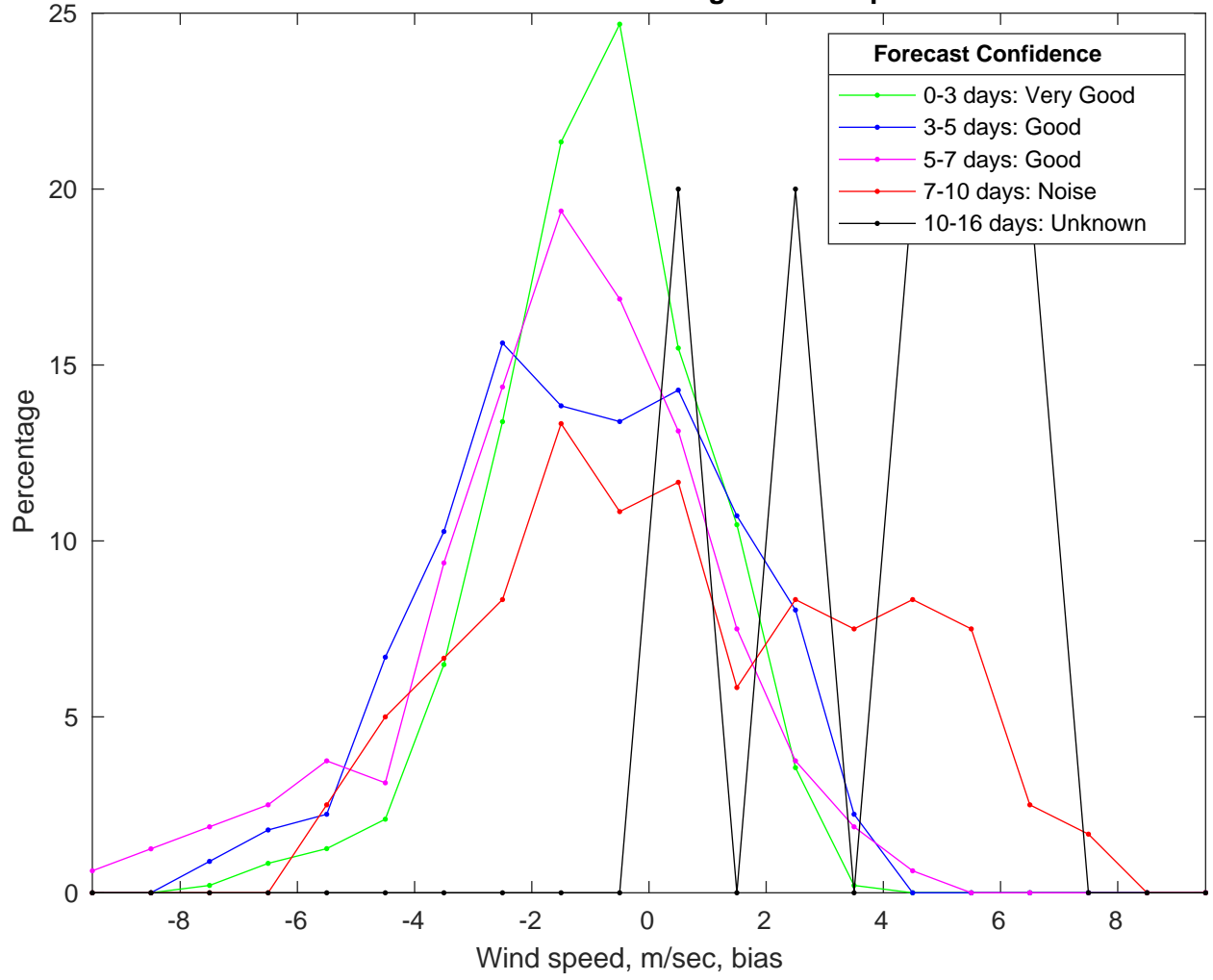
NDBC 42040 vs GFS Winds Bias Histogram: 19-Sep-2024
