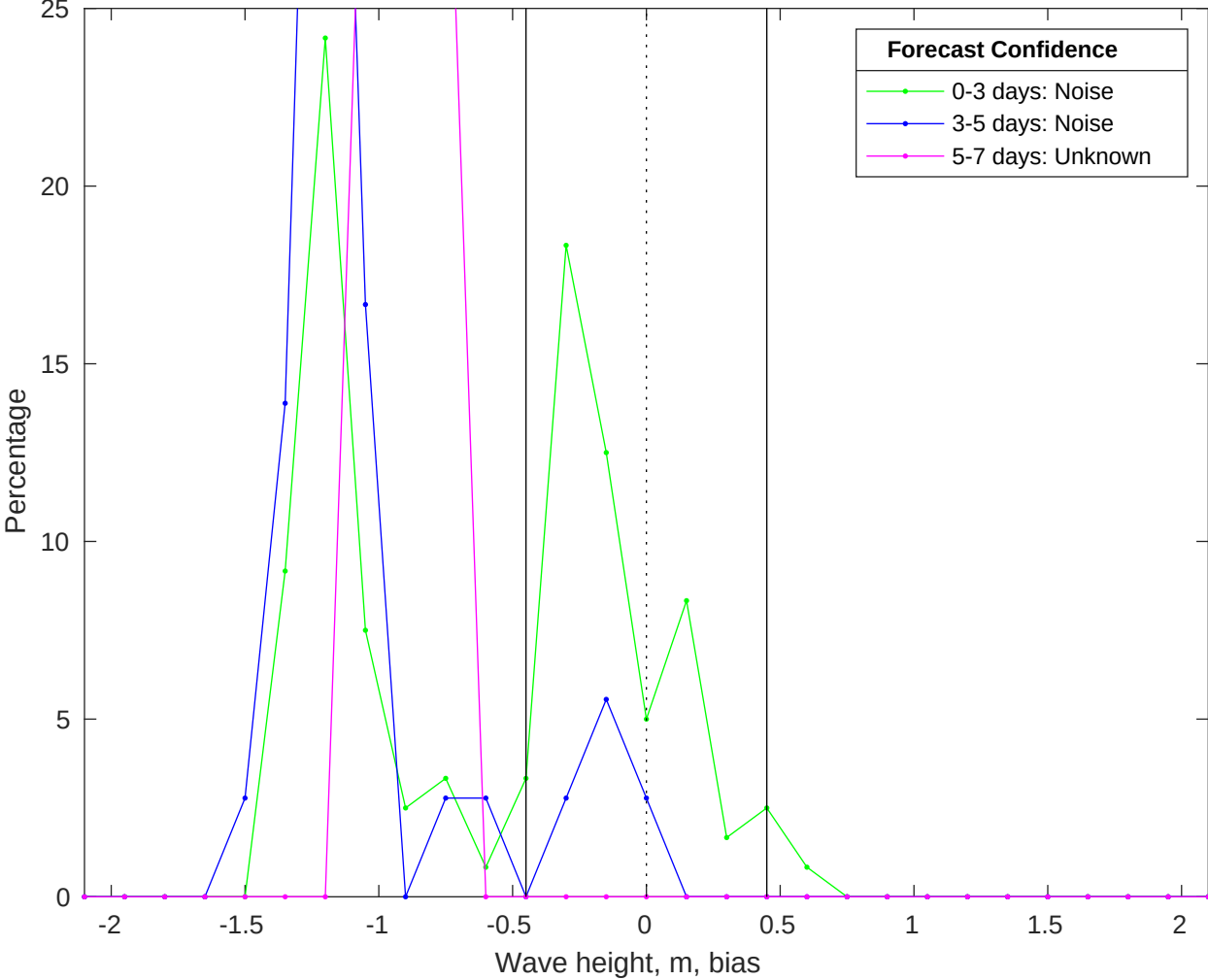
NDBC 42058 vs CMEMS Waves Bias Histogram: 29-Jan-2026
