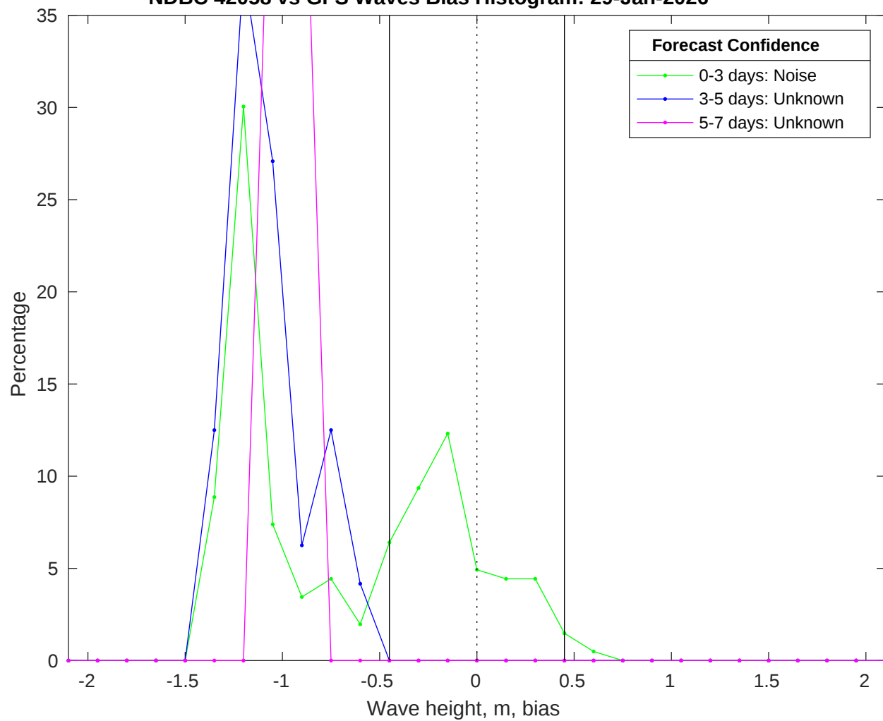
NDBC 42058 vs GFS Waves Bias Histogram: 29-Jan-2026
