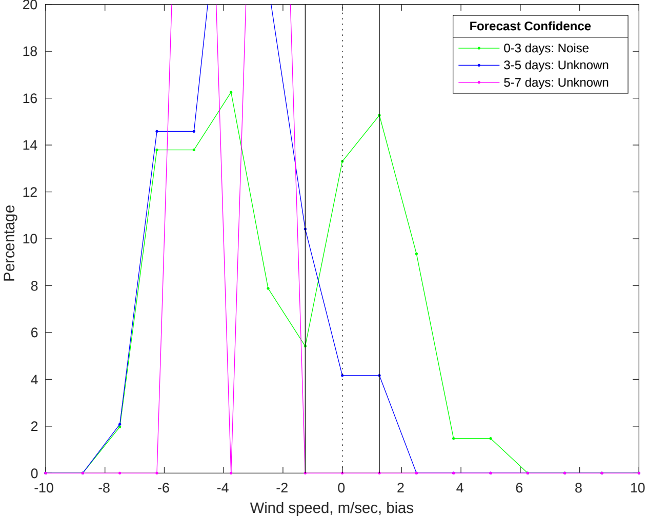
NDBC 42058 vs GFS Winds Bias Histogram: 29-Jan-2026
