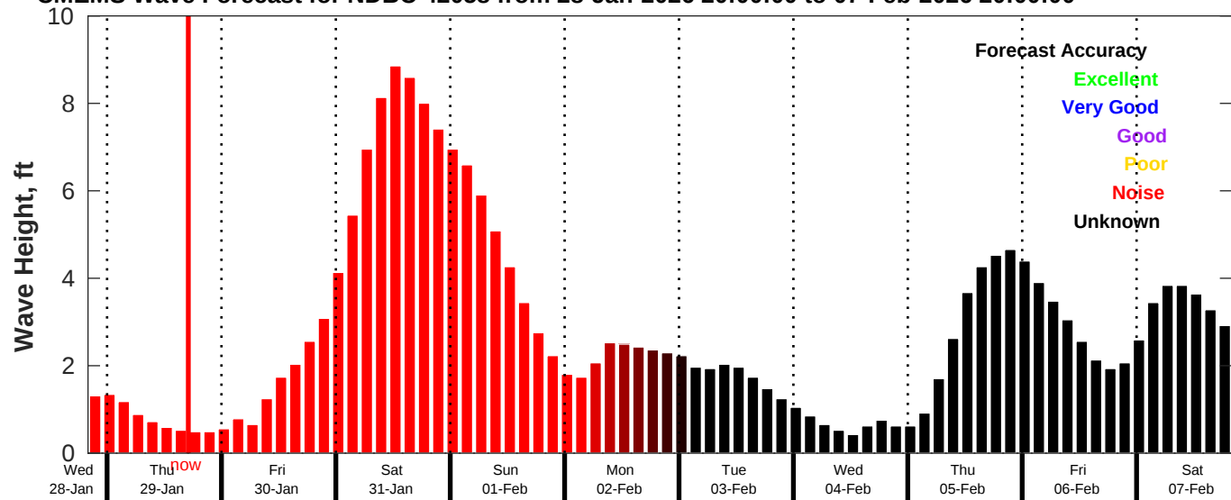
CMEMS Wave Forecast for NDBC 42058 from 28-Jan-2026 20:00:00 to 07-Feb-2026 20:00:00
