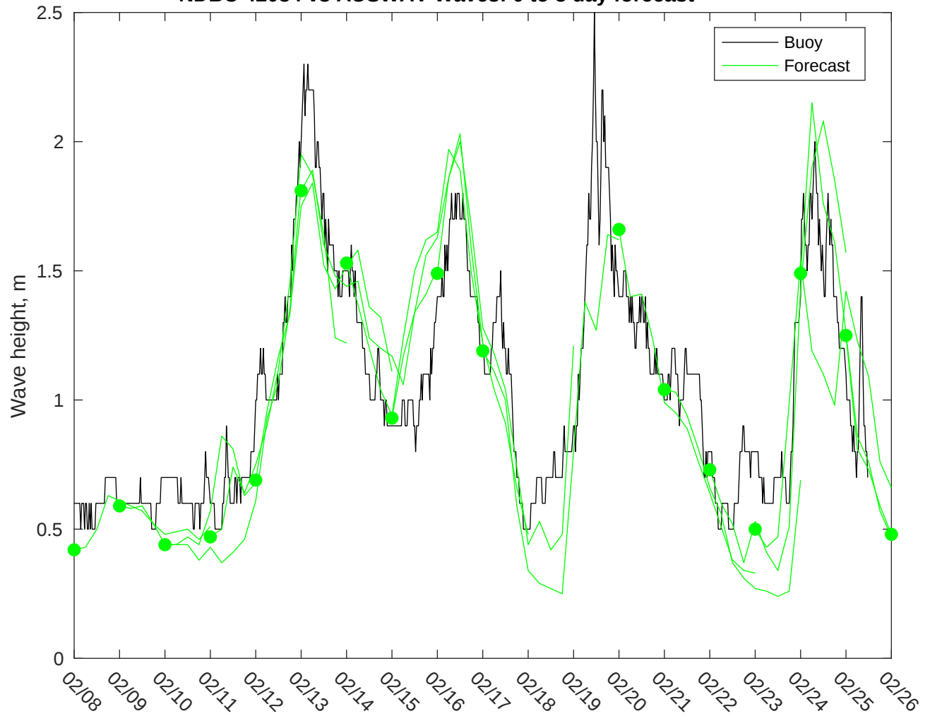
NDBC 42084 vs AUSWAV Waves: 0 to 3 day forecast
