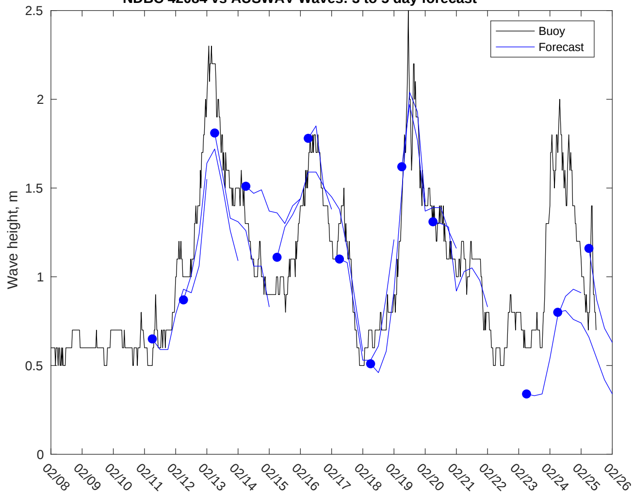
NDBC 42084 vs AUSWAV Waves: 3 to 5 day forecast
