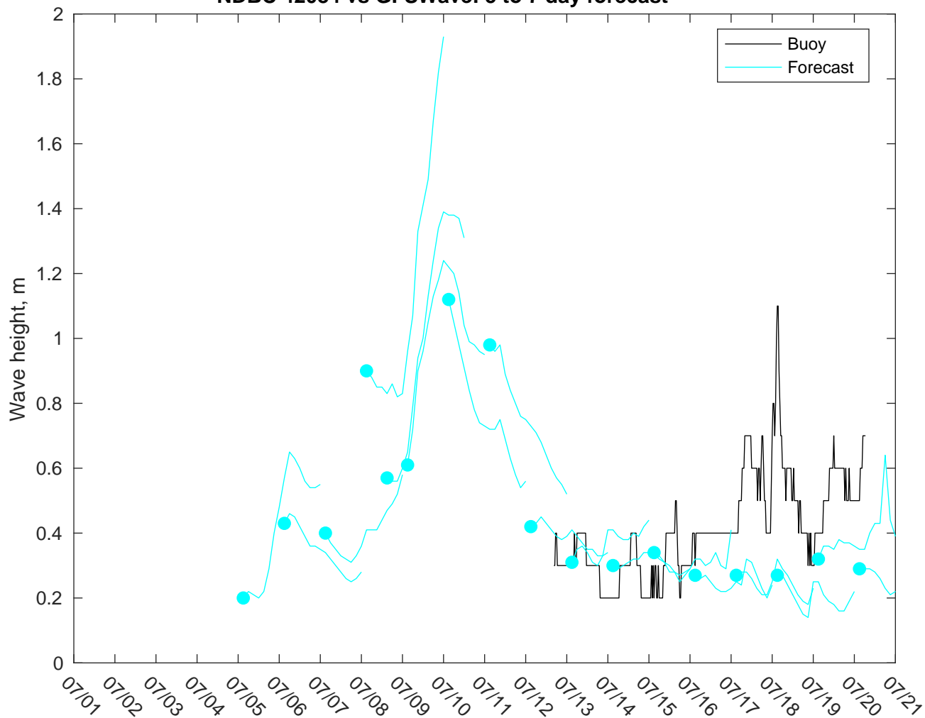
NDBC 42084 vs GFSWave: 5 to 7 day forecast
