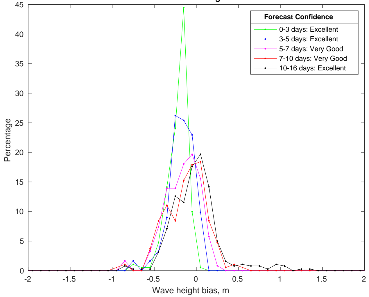
NDBC 42084 vs GFSWave Bias Histogram: 20-Jul-2024
