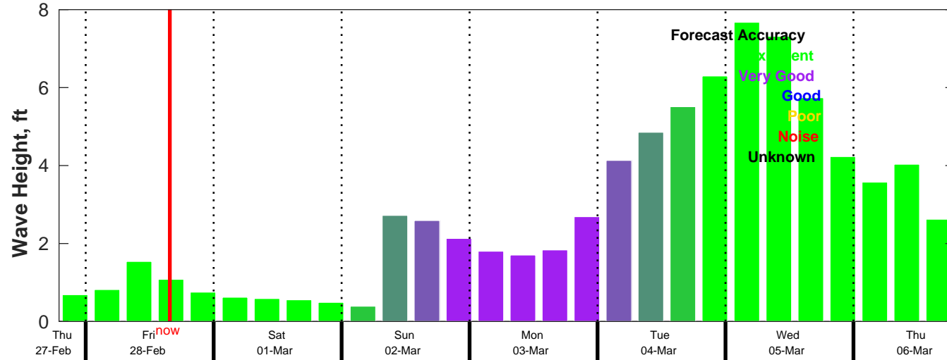
AUSWAV Wave Forecast for NDBC 42084 from 27-Feb-2025 19:00:00 to 06-Mar-2025 19:00:00
