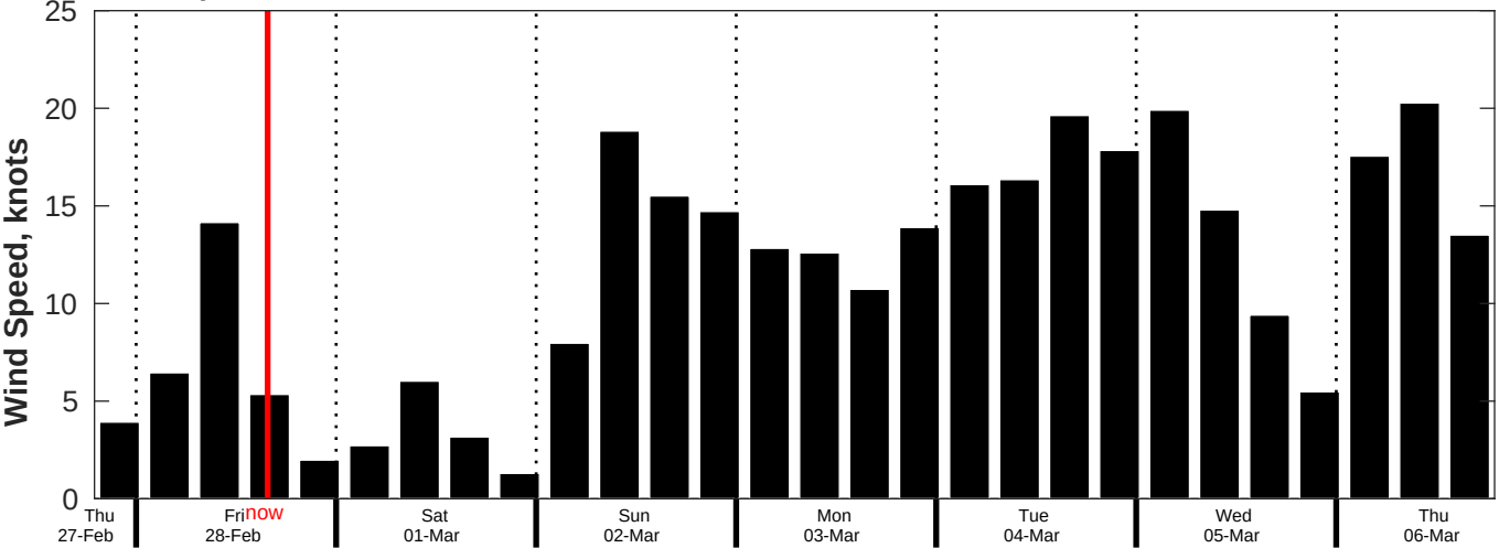
AUSWAV Wind Speed Forecast for NDBC 42084 from 27-Feb-2025 19:00:00 to 06-Mar-2025 19:00:00
