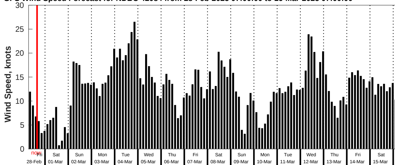
GFS Wind Speed Forecast for NDBC 42084 from 28-Feb-2025 07:00:00 to 16-Mar-2025 07:00:00
