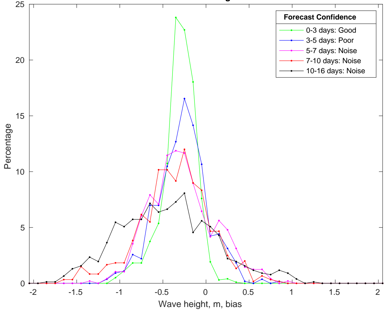
NDBC 42084 vs GFSWaves Bias Histogram: 12-Dec-2024
