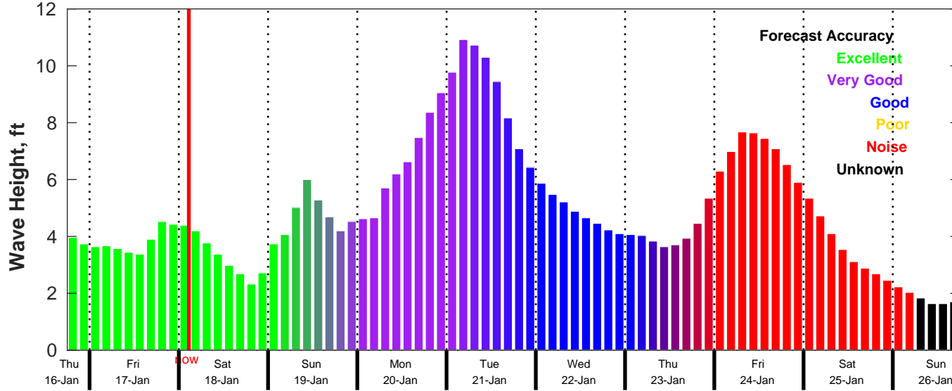
CMEMS Wave Forecast for NDBC 42092 from 16-Jan-2025 18:00:00 to 26-Jan-2025 18:00:00
