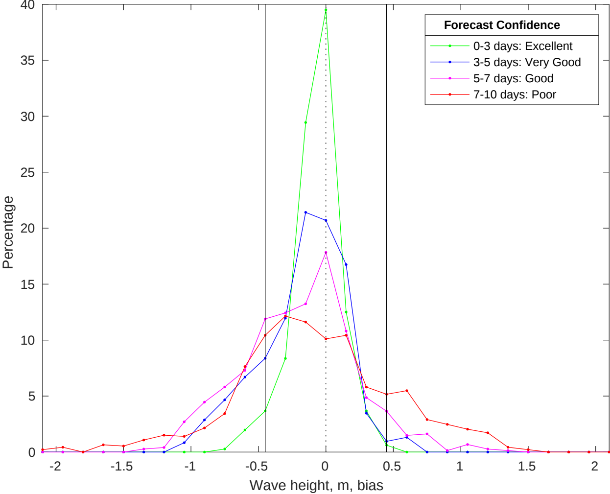
NDBC 44008 vs CMEMS Waves Bias Histogram: 03-Oct-2025
