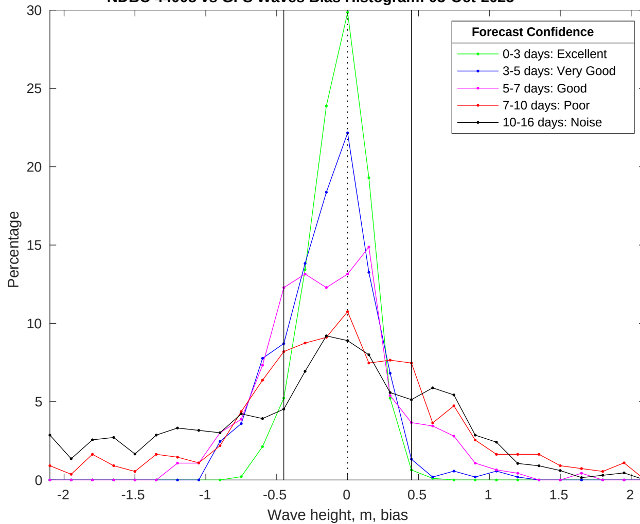
NDBC 44008 vs GFS Waves Bias Histogram: 03-Oct-2025
