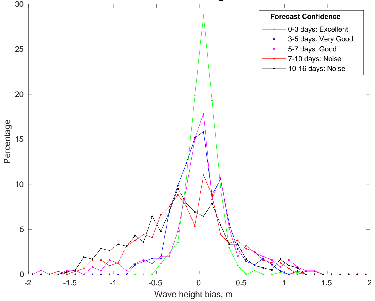
NDBC 44008 vs GFSWave Bias Histogram: 20-Jul-2024
