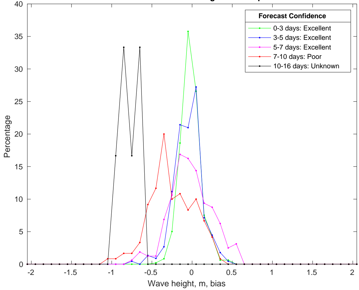
NDBC 44008 vs GFSWaves Bias Histogram: 19-Sep-2024
