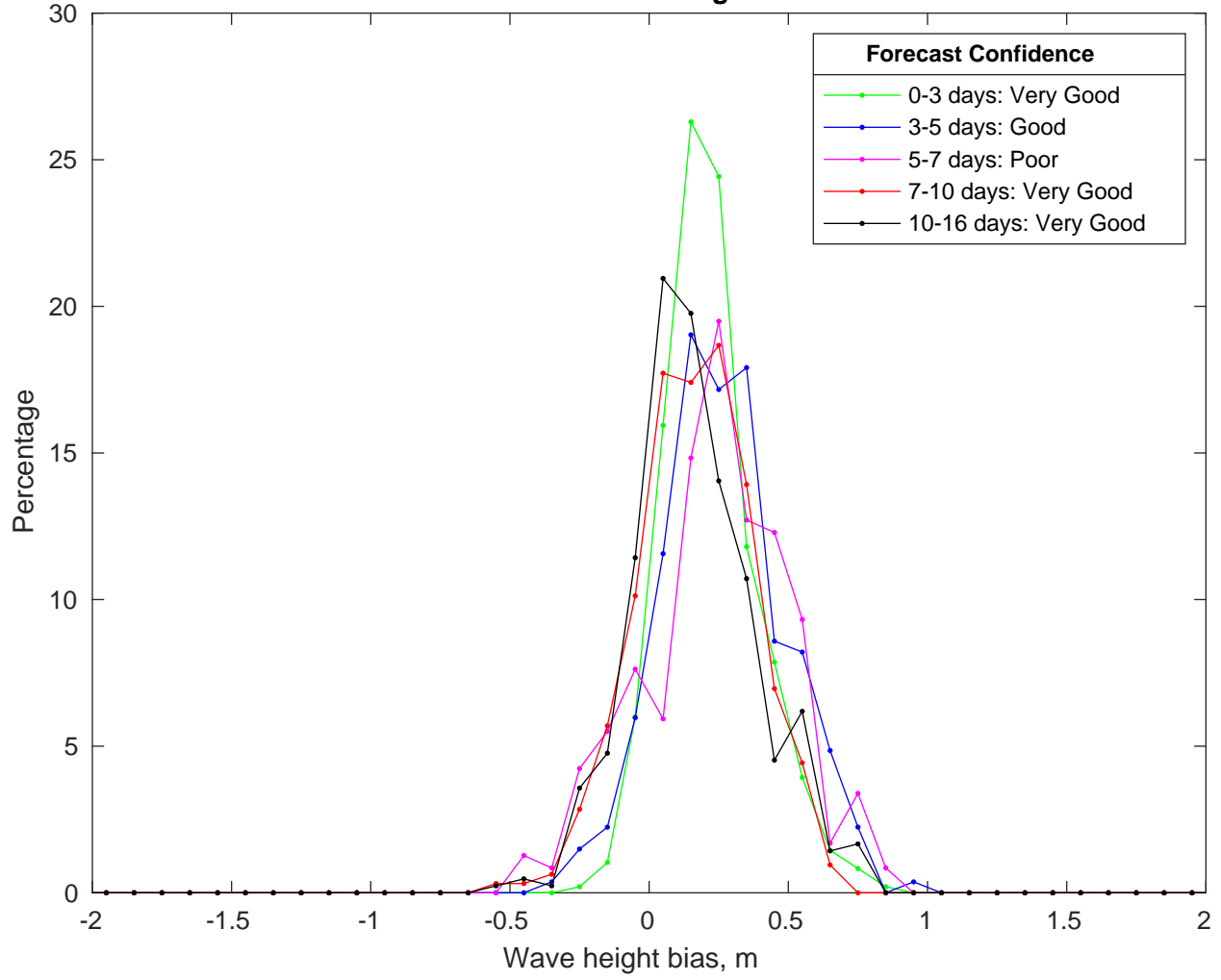
NDBC 44020 vs GFSWave Bias Histogram: 20-Jul-2024
