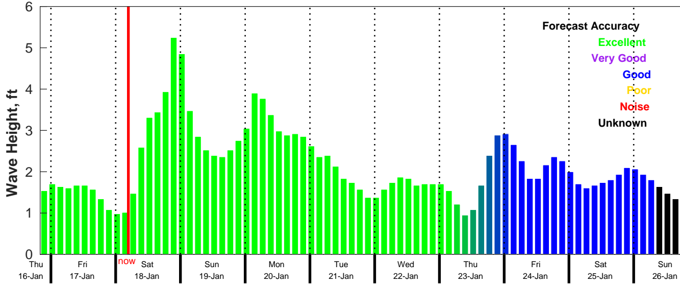
CMEMS Wave Forecast for NDBC 44020 from 16-Jan-2025 20:00:00 to 26-Jan-2025 20:00:00
