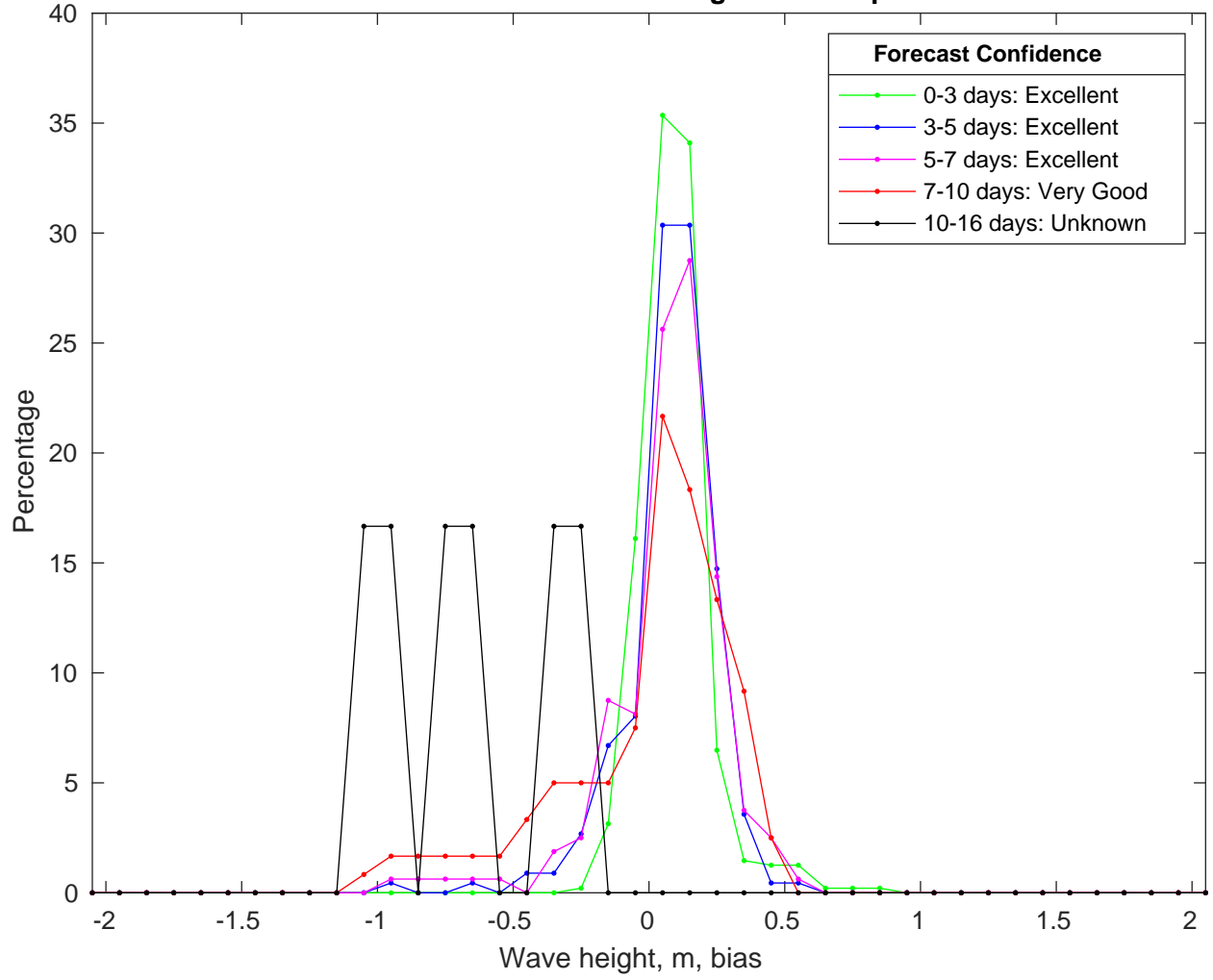
NDBC 44020 vs GFSWaves Bias Histogram: 19-Sep-2024
